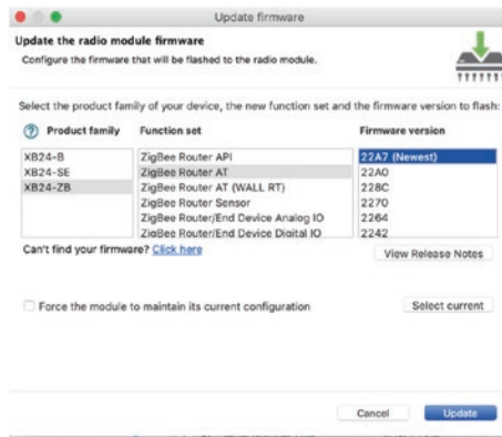
Figure 2-19. Choose the firmware (series 2.5 and older)
