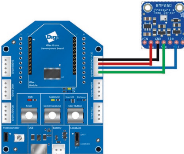
Figure 4-10. Connecting the BMP280 breakout board using Grove to jumper wire cable
