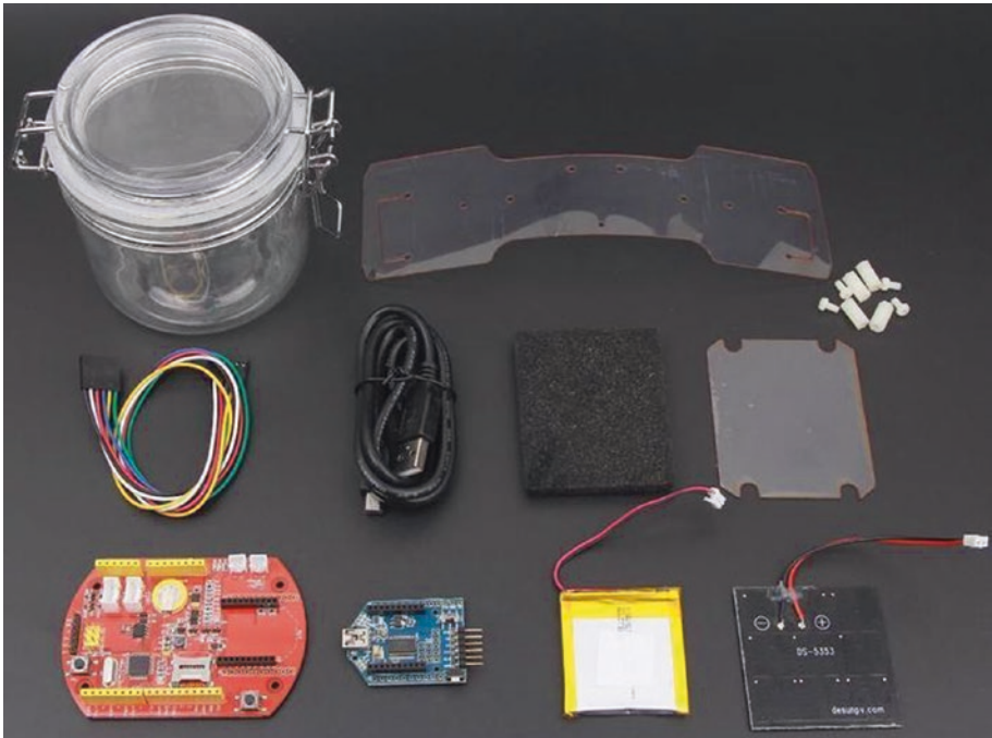
Figure 11-2. Seed Studio Stalker wireless sensor node (courtesy of Seed Studio)
