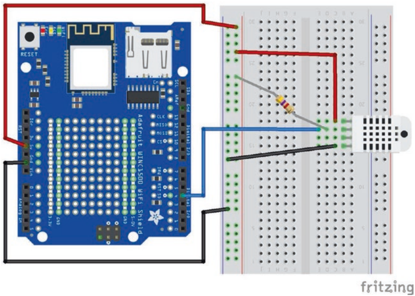
Figure 9-7. Wiring the DHT22
