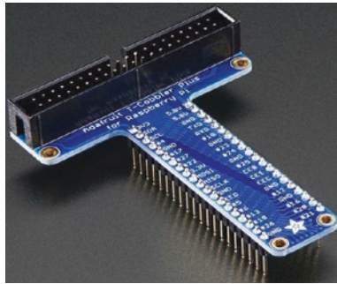
Figure 5-12. Pi T-Cobbler Plus breakout board (courtesy of Adafruit)
