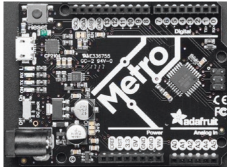
Figure 6-15. Metro 328 (courtesy of Adafruit)
