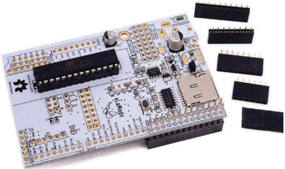
Figure 11-4. Raspberry Pi Alamode (courtesy of Seed Studio)
