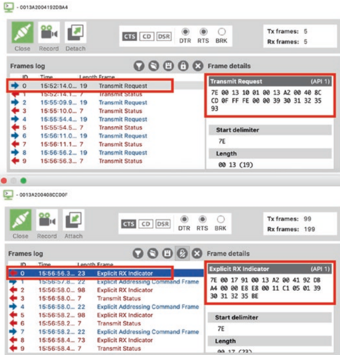
Figure 2-40. Frame sent and received
