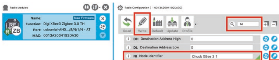
Figure 2-15. Change the name identifier for a module
