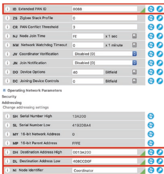
Figure 2-31. Configuring the coordinator
