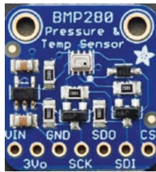
Figure 5-16. BMP280 I2C sensor (courtesy of Adafruit)
