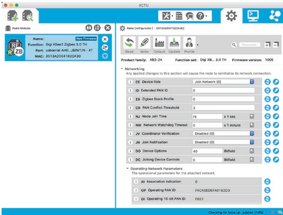
Figure 2-14. XCTU radio module settings
