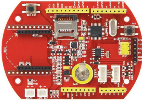
Figure 11-3. Seeeduino Stalker Arduino-compatible board (courtesy of Seeed Studio)
