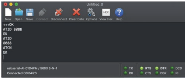
Figure 2-24. Configuring a module (AT mode) using CoolTerm
