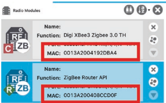
Figure 2-30. Identifying the 64-bit address using XCTU
