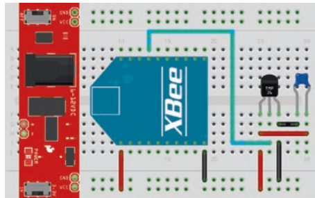
Figure 5-19. XBee sensor node
