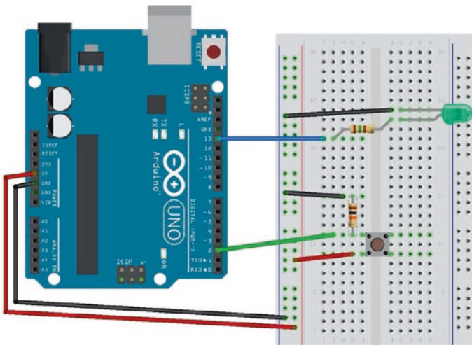
Figure 6-19. Diagram of an LED with a pushbutton
