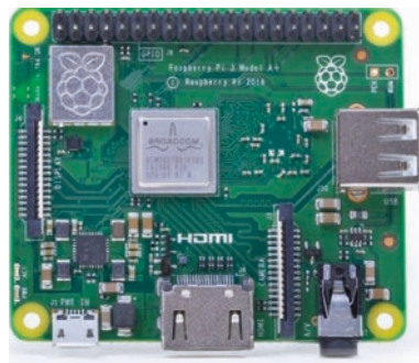
Figure 5-1. Raspberry Pi 3A+ (courtesy of the Raspberry Pi Foundation)
