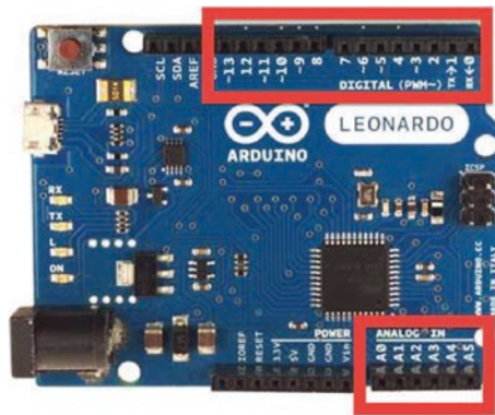
Figure 6-20. Identifying the I/O pins on an Arduino board
