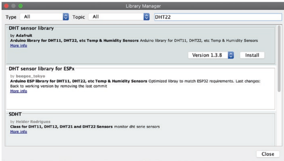
Figure 9-8. Library manager
