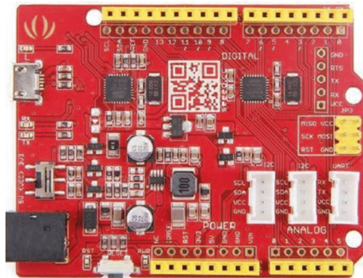
Figure 6-11. Seeeduno (courtesy of Seeed Studio)
