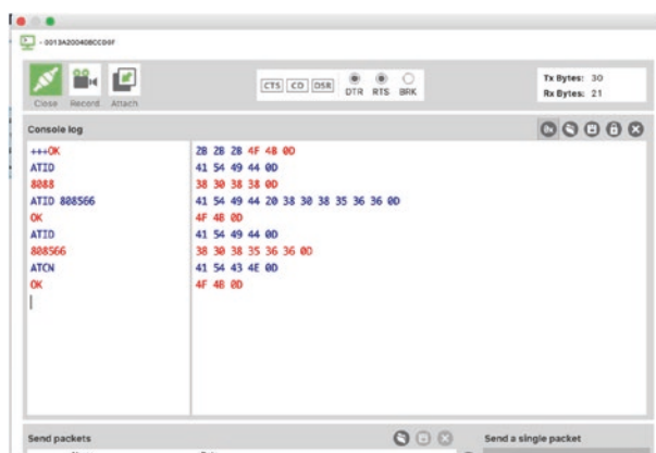
Figure 2-23. Configuring a module (AT mode) in a console
